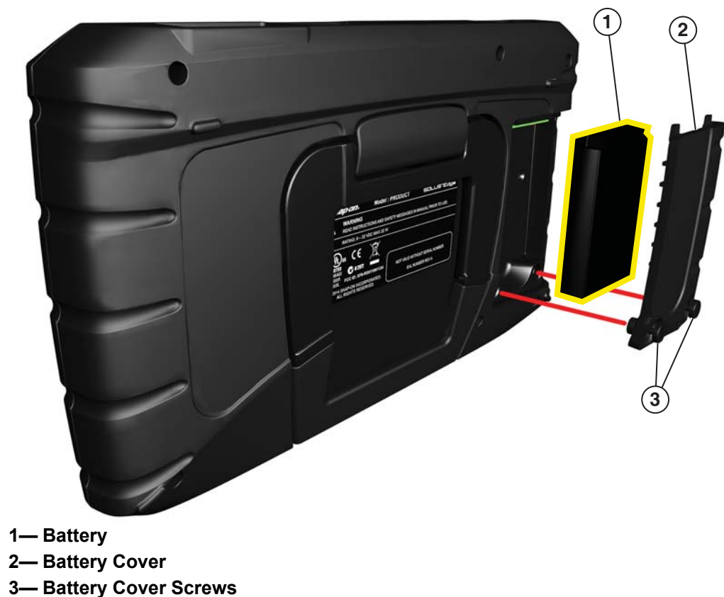
Figure 10-1 Battery pack location
